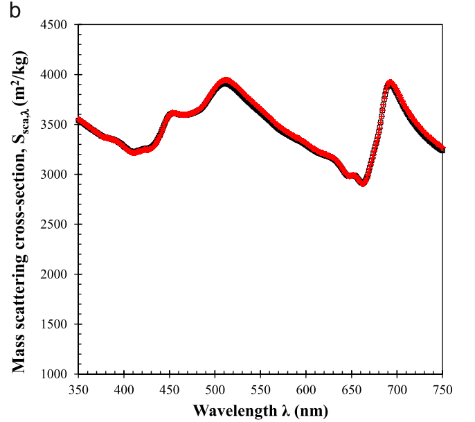
Fig. 5. Directly measured average spectral mass absorption \bar{A}_{abs,\lambda} and scattering \bar{S}_{sca,\lambda} cross-sections of C. vulgaris suspensions between 350 and 750 nm for biomass concentrations X of 0.035 and 0.049 g/L.
