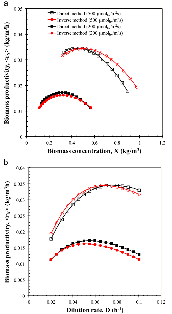
Fig. 9. Comparison of biomass productivity \langle r_X \rangle of C. vulgaris grown in a 1 cm thick flat-plate PBRs exposed to 200 or 500 \mu\text{mol}_{h\nu}/\text{m}^2 \text{ s} incident white LED light, predicted using Eqs. (12)–(16) as a function of either (a) the steady-state biomass concentration X or (b) the dilution rate D . The predictions used the radiation characteristics obtained from either direct measurements or retrieved by the inverse method.
