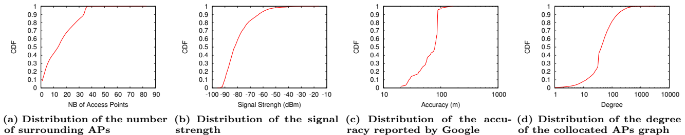
Figure 3: Cumulative Distribution Functions.
