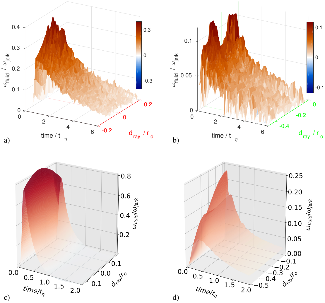
Figure 10. Color surface rendering of the fluid angular velocity \omega_{fluid} , as a function of time (normalized by t_\eta ) and distance along the ray (normalized by r_o ), with d_{ray} = 0 at the midpoint of the ray. Angular velocities are normalized by \Delta\varphi/t_{jerk} . (a) Ray 1. Stack of 5 records for f = 0 . (b) Ray 2. Stack of 8 records for f = -10 Hz. (c) Ray 1. Synthetics for f = 0 , with the same parameters as in figure 5c. (d) Ray 2. Synthetics for f = -10 Hz.
