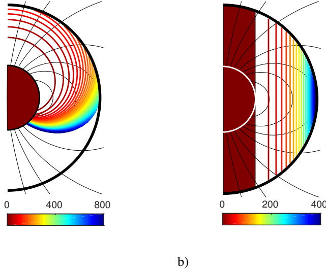
Figure 3. Wavefronts of (a) ideal Alfvén waves and (b) ideal torsional Alfvén waves in a dipolar magnetic field. The waves are triggered by a jerk of the inner sphere (in brown). The color scales give the travel times in milliseconds for the DTS- \Omega parameters.
