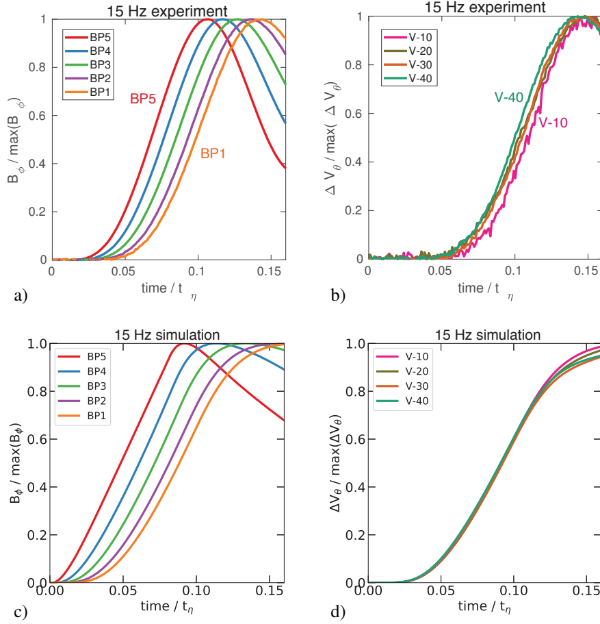
Figure 4. Magnetic and electric waveforms of torsional Alfvén waves in the DTS- \Omega experiment for a rotation rate f = 15 Hz. Observed (a) and simulated (c) B_\varphi azimuthal magnetic signals inside the liquid at a latitude of -20^\circ for five radii color-coded as in Figure 1b. Observed (b) and simulated (d) \Delta V_\theta electric potential differences at the surface of the stainless steel outer shell at four latitudes. All signals are normalized to their maximum amplitude, and plotted versus time normalized by the magnetic diffusion time t_\eta .
