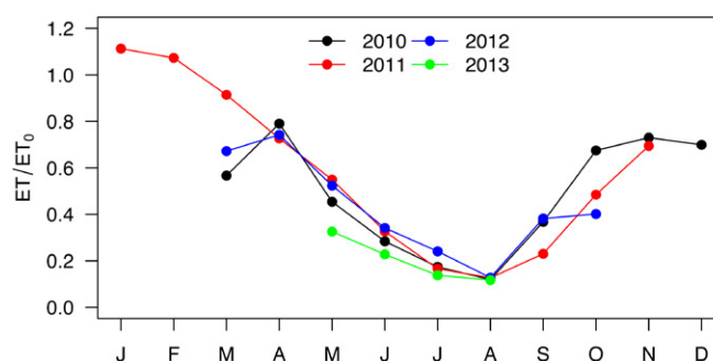
Fig. 7. Seasonal evolution of the ratio of actual (ET) to reference ( ET_0 ) evapotranspiration at the hillslope scale across 4 yr in Kamech. Actual evapotranspiration was measured by the flux tower installed on the northern hillslope of Kamech, whereas ET_0 was measured by the meteorological station (adapted from Zitouna-Chebby et al., 2018).
