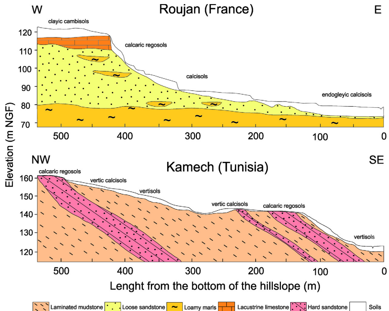
Fig. 3. Geological cross-sections of the main hillslope of the two catchments. The main soils are described according to the World Reference Base classification (IUSS Working Group WRB, 2014).
