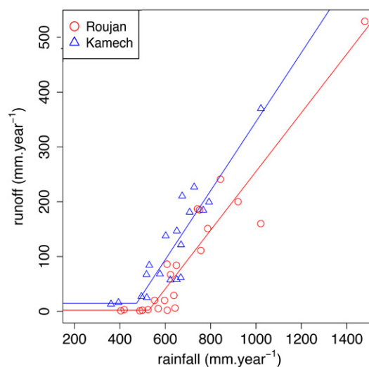
Fig. 2. Relationship between annual rainfall and annual stream runoff in the two sites. The period ranges from 1993 to 2015 in Roujan and from 1995 to 2013 in Kamech (adapted from Voltz et al., 2016).
