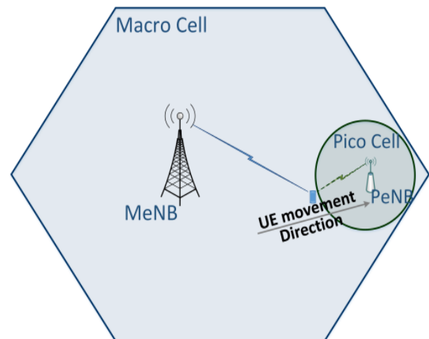
Fig. 1: High-level handover architecture
