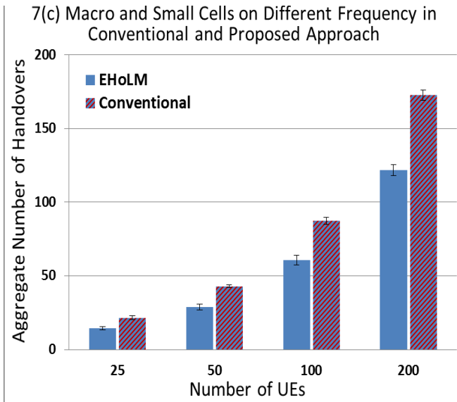
Fig. 7. Number of handovers with respect to number of UEs
