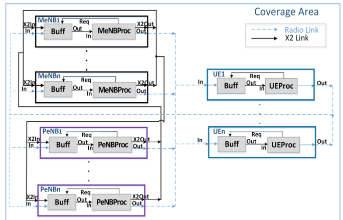
Fig. 5. Simplified DEVS model for CoMP control architecture
