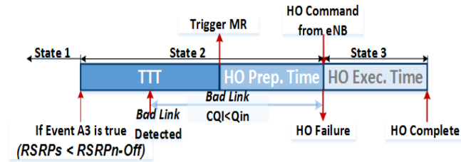
Fig. 2: Block diagram of handover states
