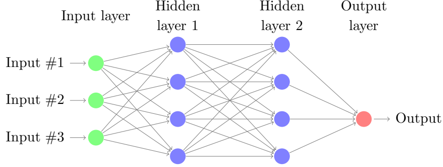
Figure 1: Representation of a neural network with d = 3 , 2 hidden layers, d_1 = d_2 = 4 , d_3 = 1 .
