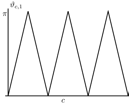
Figure 2: The angle \vartheta_{c, \alpha} as a function of c for \alpha = 1 .
