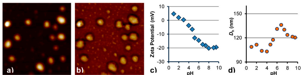
Figure 3. AFM (a) height and (b) phase images for MPIC micelles G1@Fe 3 O 4 @PAA 27 - b -PHEA 260 at f = 0.5 . The scale of the AFM images is 500 \times 500 nm 2 . (c) Zeta potential and (d) Intensity-weighted hydrodynamic diameter D_h of mentioned MPIC micelles as a function of pH.
