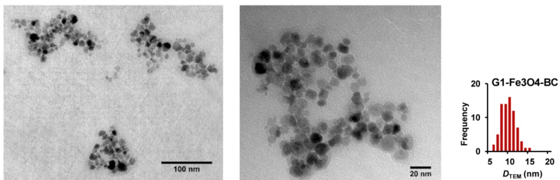
Figure S1-4. TEM images of MPIC micelles showing Fe 3 O 4 crystallites in G1@Fe 3 O 4 @PAA 27 - b -PHEA 260 f = 0.5 .
