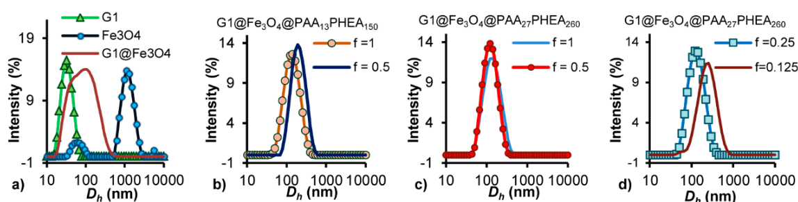
Figure 1. Hydrodynamic size distribution for (a) G1 (pH 4), Fe 3 O 4 (pH 1.4) and G1@Fe 3 O 4 (pH 1.4). (b–d) MPIC micelles G1@Fe 3 O 4 @PAA- b -PHEA (pH 7) for different f ratios at 25 °C.
