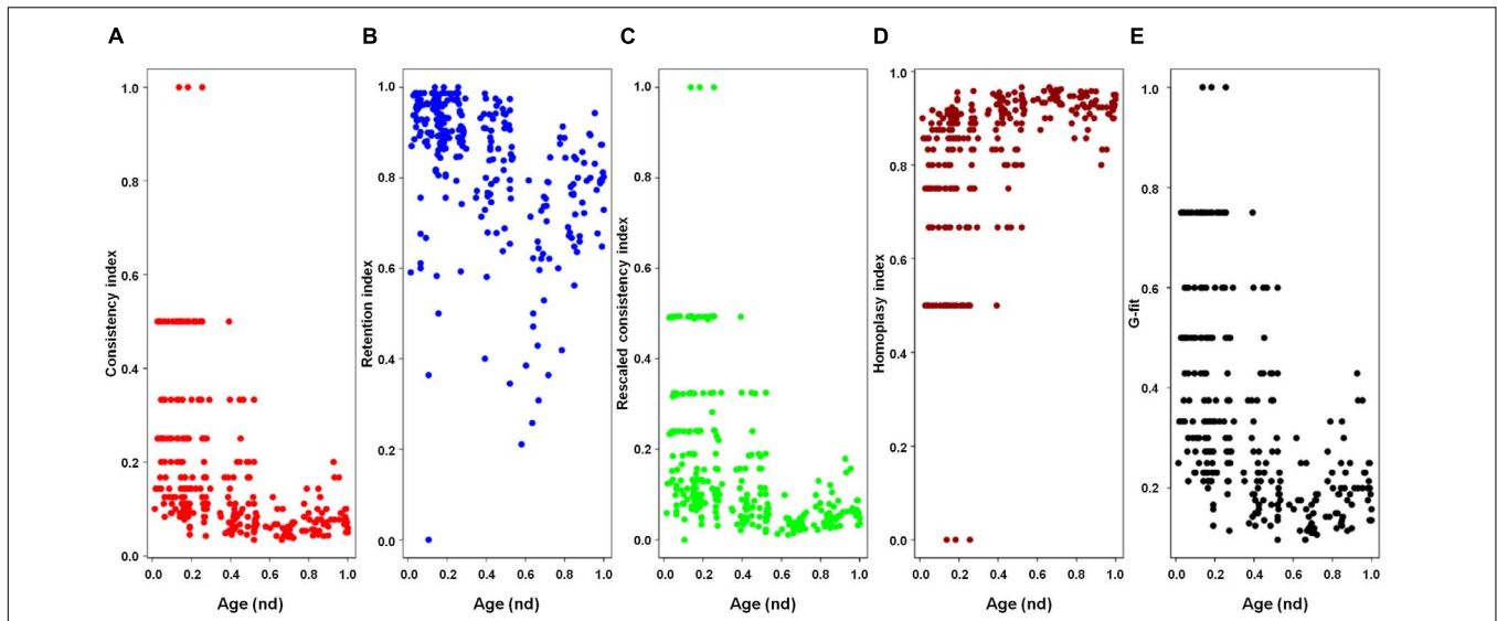
FIGURE 4 | Plots of the indices of the phylogenetic tree of proteomes describing the evolution of 182 proteomes randomly sampled from cellular organisms and viruses (corresponding to Figure 2 ) against the age of the phylogenetic character [fold superfamily (FSF)]. Five measures of the levels of lateral sequence transfers for the maximum parsimony tree reconstruction performed in the present study, namely consistency index (A) , retention index (B) , rescaled consistency index (C) , homoplasy index (D) , and G-fit (E) , are plotted against the age of the phylogenetic character FSF [measured as node distance ( nd ) values] for 289 characters (FSF) shared by archaea, bacteria, eukaryota, and viruses. High retention indices, especially for lower nd values (corresponding to older domains), indicates excellent fit of the characters to the phylogeny.
