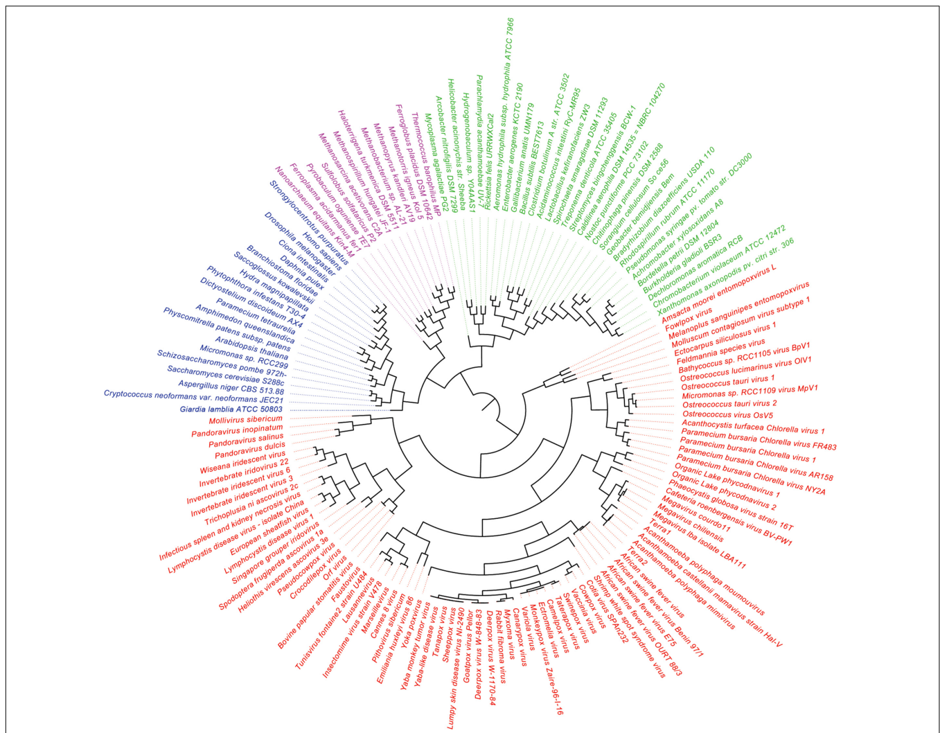
FIGURE 8 | Hierarchical clustering by phyletic pattern based on the presence/absence of informational Clusters of Orthologous Groups (COGs) of proteins. The Megavirales members are represented in red, Bacteria members in green, Archaea members in pink, and Eukarya members in blue.
