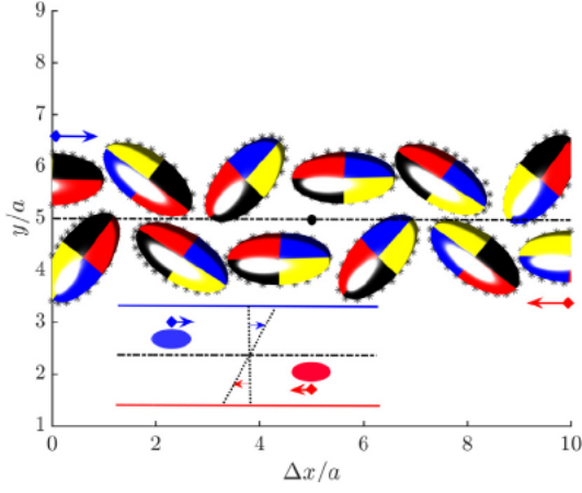
Fig. 2. Time sequence of two moving prolate spheroids with Ar = 2 within the shear-gradient plane for initial orientations \varphi_0 = \pi/2 and \theta_0 = 0 . Asterisks show the ellipsoid surface from Pozrikidis (2006), four colors and solid line show FCM results. (For interpretation of the references to color in this figure legend, the reader is referred to the web version of this article.)
