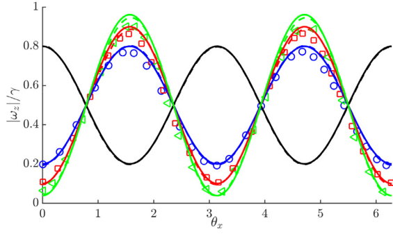
Fig. 6. Instantaneous angular velocity along the vorticity vector in a shear flow for spheroid (oblate Ar = 0.5 and prolate Ar = 2 - 5 ) in a suspension with volume fraction \phi = 0.058 . --- FCM at Re_p = 0.1 compared with — Stokes solution of Jeffery. Colors distinguish four aspect ratios. Black: Ar = 0.5 , blue: Ar = 2 , red: Ar = 3 and green: Ar = 5 . Symbols are results from Daghooghi and Borazjani (2015) at Re_p = 0.01 where \circ : Ar = 2 , \square : Ar = 3 and \triangle : Ar = 5 . (For interpretation of the references to color in this figure legend, the reader is referred to the web version of this article.)
