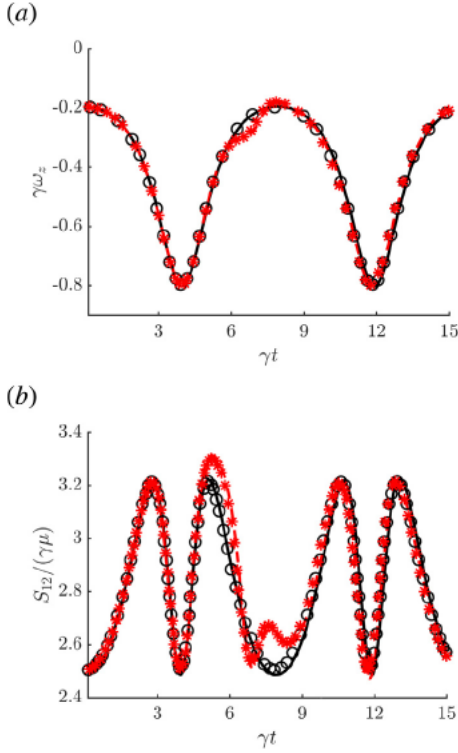
Fig. 3. Evolution of the rotation rate and the shearing component of the particle stress tensor during particle interception for \varphi_0 = \pi/2 and \theta_0 = 0 . (a) the rate of rotation around the z axis; (b) particle stress tensor. — FCM for an isolated spheroid; - - FCM for pair of spheroids during interception; circle stands for an isolated spheroid and asterisks show the results for a pair of spheroids in Pozrikidis (2006).
