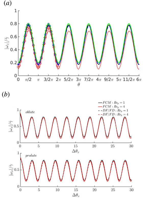
Fig. 7. Effect of the Reynolds number on the instantaneous angular velocity ( \omega_x = d\theta/dt ). (a): a prolate spheroid ( Ar = 2 ) about the vorticity vector in a shear flow. The volume fraction is \phi = 0.058 . — Jeffery orbit. FCM: — Re_p = 0.1 , - - - Re_p = 1 and . . . . Re_p = 10 . Symbols are results from Daghooghi and Borazjani (2015) where + : Re_p = 0.1 , * : Re_p = 1 and \circ : Re_p = 10 ; (b) is the comparison between FCM (line) and DF/FD (dash line); the top panel shows the symmetry axis of an oblate spheroid ( Ar = 0.5 ) rotating about the vorticity vector at two Reynolds numbers, black is Re_p = 1 and red is Re_p = 4 ( Re_p is based on its semi-major axis). The bottom panel shows the symmetry axis of a prolate spheroid ( Ar = 2 ) rotating about the vorticity vector. (For interpretation of the references to color in this figure legend, the reader is referred to the web version of this article.)
