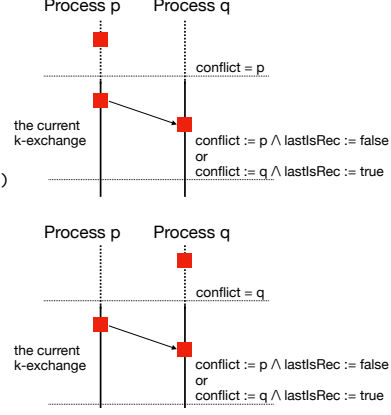
Fig. 10: The monitor \mathcal{M}_{viol}(k) . \mathbb{B} is the set of Booleans and \mathbb{N} is the set of natural numbers. Initially, conflict is \perp , while lastIsRec and sawRS are false .
