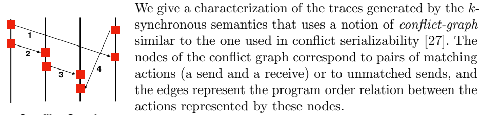
Conflict Graph:
