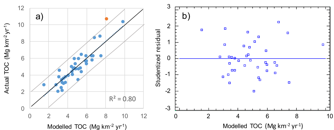
Figure 2. (a) Scatterplot between modelled and actual TOC export data, with the 95% prediction intervals for new observations given in grey lines around 1:1 line in black color; (b): Studentized residual versus predicted TOC export values.
