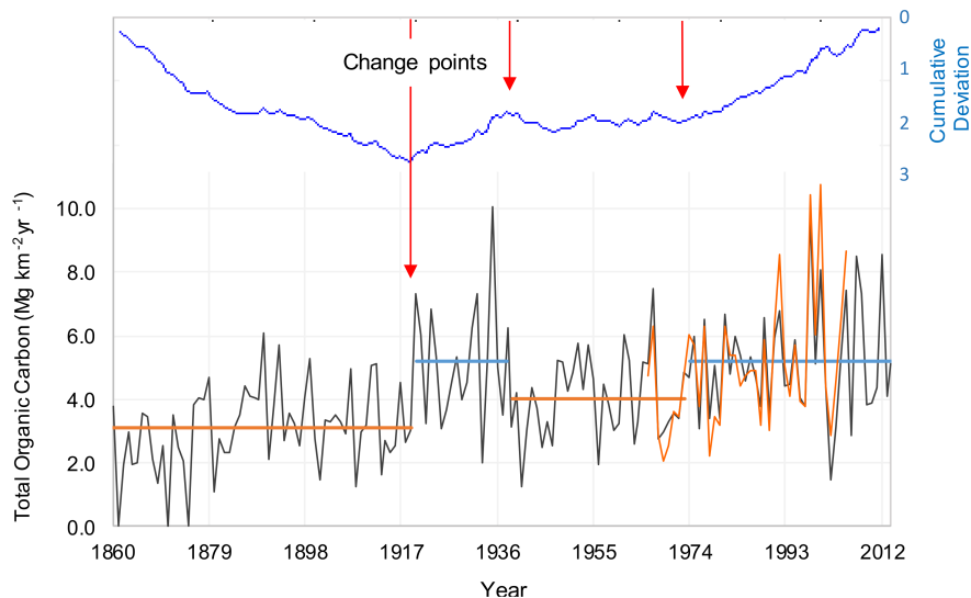
Figure 3. Simulated TOC export by model (Equation (2)) in \text{Mg km}^{-2} \text{ year}^{-1} from Simojoki basin during the period 1860–2014, with change points (arrows). The intermittent intervals with high TOC export (blue lines) and low TOC export (orange lines) were identified by the Buishand test (blue curve). Two histogram plots are also reported for the recent period. Orange curve represents the actual TOC for the period of available data at end series.
