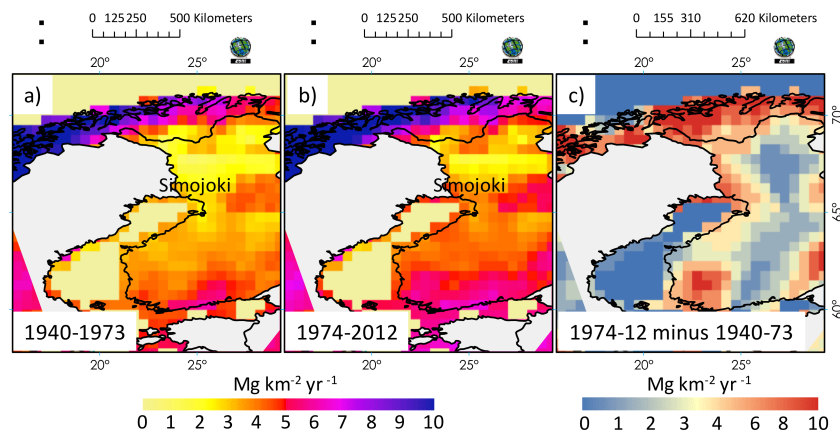
Figure 4. Total C export for each grid-cell ( 2500 \text{ km}^2 ) across Finnish and northern Scandinavian areas. (a) for 1940–1973; (b) for 1974–2012; (c) relative differences 1974–2012 minus 1940–1973 (arranged from CRU-TS3.22 precipitation, via Map Calculator function within ESRI-ArcGIS, http://www.esri.com/software/arcgis ).
