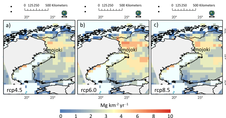
Figure 5. TOC export anomalies across Finnish and northern Scandinavian areas deriving from CMIP5 mean scenario runs 2021–2050 minus 1974–2012, for RCPs 4.5, 6.0 and 8.5, respectively.
