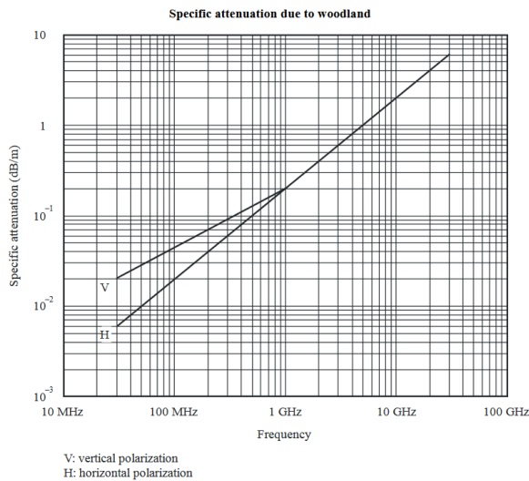
Figure 9 : Vegetation attenuation [18]
