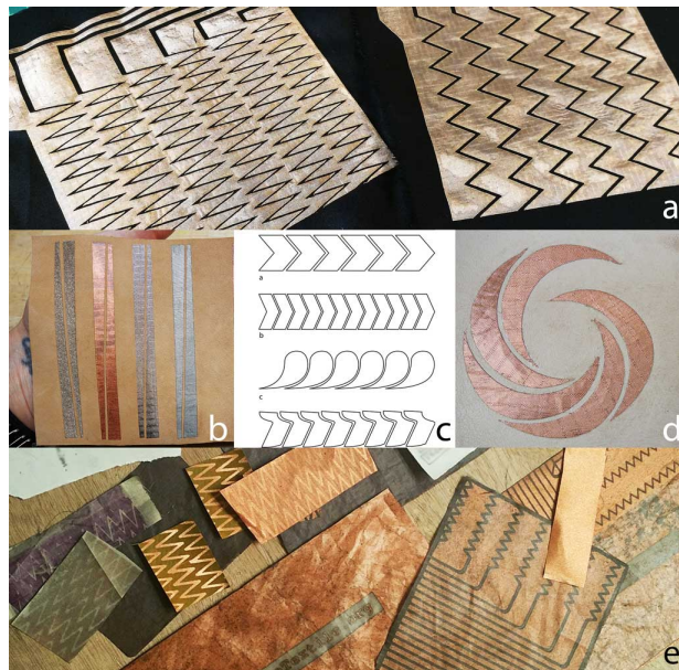
Figure 1 - a) Electrodes of two sensors used in this paper b) capacitive sliders by Rachel Freire c, d) electrode designs and circular slider by Kobakant e) electrode testing samples at Datapalette
