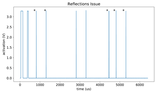
Figure 7: Reflections off the walls cause undesired pulses (asterisk) in the photodiode signal (compare to Figure 4).
