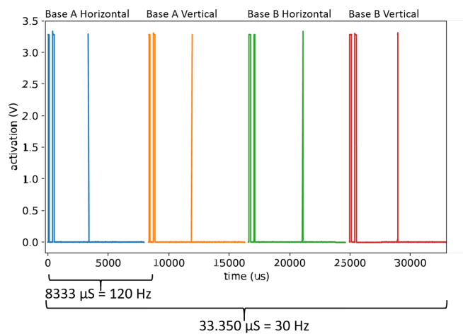
Figure 4: Light signal sequences (4 are shown): wide pulses are base station flashes and short pulses are laser plane scans.
