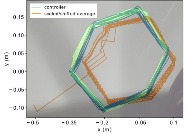
Figure 6: Accuracy comparison between commercial controller and Hive Tracker proof-of-concept in a non-ideal room. Traces from both devices are superimposed over a photo of a polygon taped to the floor. Blue = commercial controller, Orange = Hive Tracker, Green = tape on the floor.
