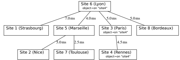
Fig. 2: Tree overlay generated from the French NREN topology, showing the location records of an object stored on Site 4.
