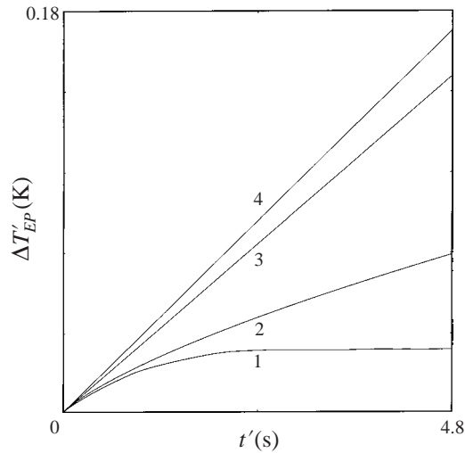
FIGURE 9. Bulk temperature variations: for g = 1 and a thermostated upper wall (curve 1), for g = 0 and a thermostated upper wall (curve 2), for g = 1 and insulated boundaries (curve 3), for g = 0 and insulated boundaries (curve 4).
