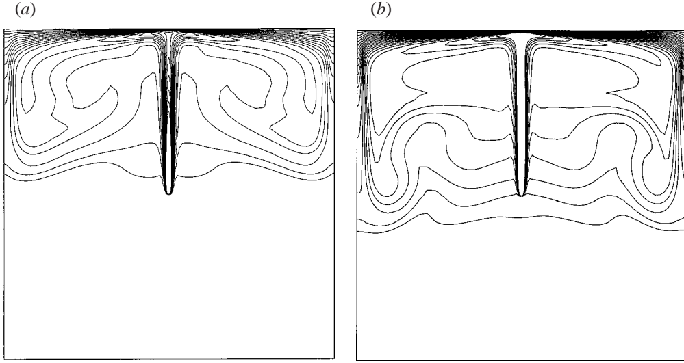
FIGURE 15. Thermal field at (a) t' = 7.14 s and (b) t' = 19 s for T'_i = T'_c + 15 K and \rho'_i = \rho'_c + 125 kg m ^{-3} .
