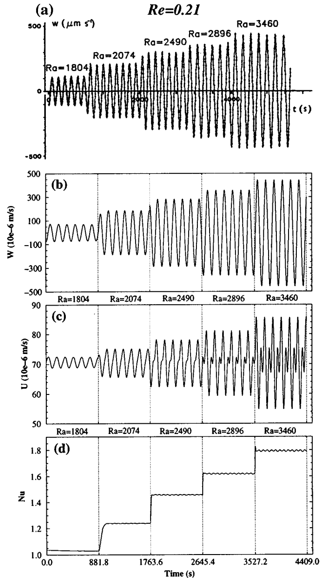
FIG. 4. Time evolution in the transversal roll phase, of the vertical [ W(t) ] and horizontal [ U(t) ] velocity components and of the space average Nusselt number [ Nu(t) ] for Re=0.21 , Ra=1804 , 2074 , 2490 , 2896 , and 3460 , and for Pr=6.4 ; (a) W(t) at (x, z) = (15.7, 0.5) from the experiments of Ouazzani et al. ; 14,16 (b),(c),(d), respectively, W(t) , U(t) , and Nu(t) at (x, z) = (7.5, 0.5) for the present numerical work ( config-1 ).
