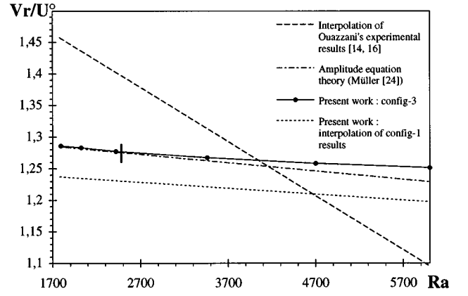
FIG. 16. Ratio of the transversal roll velocity, Vr , to the average velocity of the flow, U^\circ , as a function of Ra and for Pr=6.4 ; comparison of the numerical solutions obtained on config-1 and config-3 with the experimental results of Ouazzani et al. 14,16 and with Müller's theoretical result 24 (the limit of validity of this theory, Ra \approx 2500 , is indicated by a vertical line). All the curves are independent of Re .
