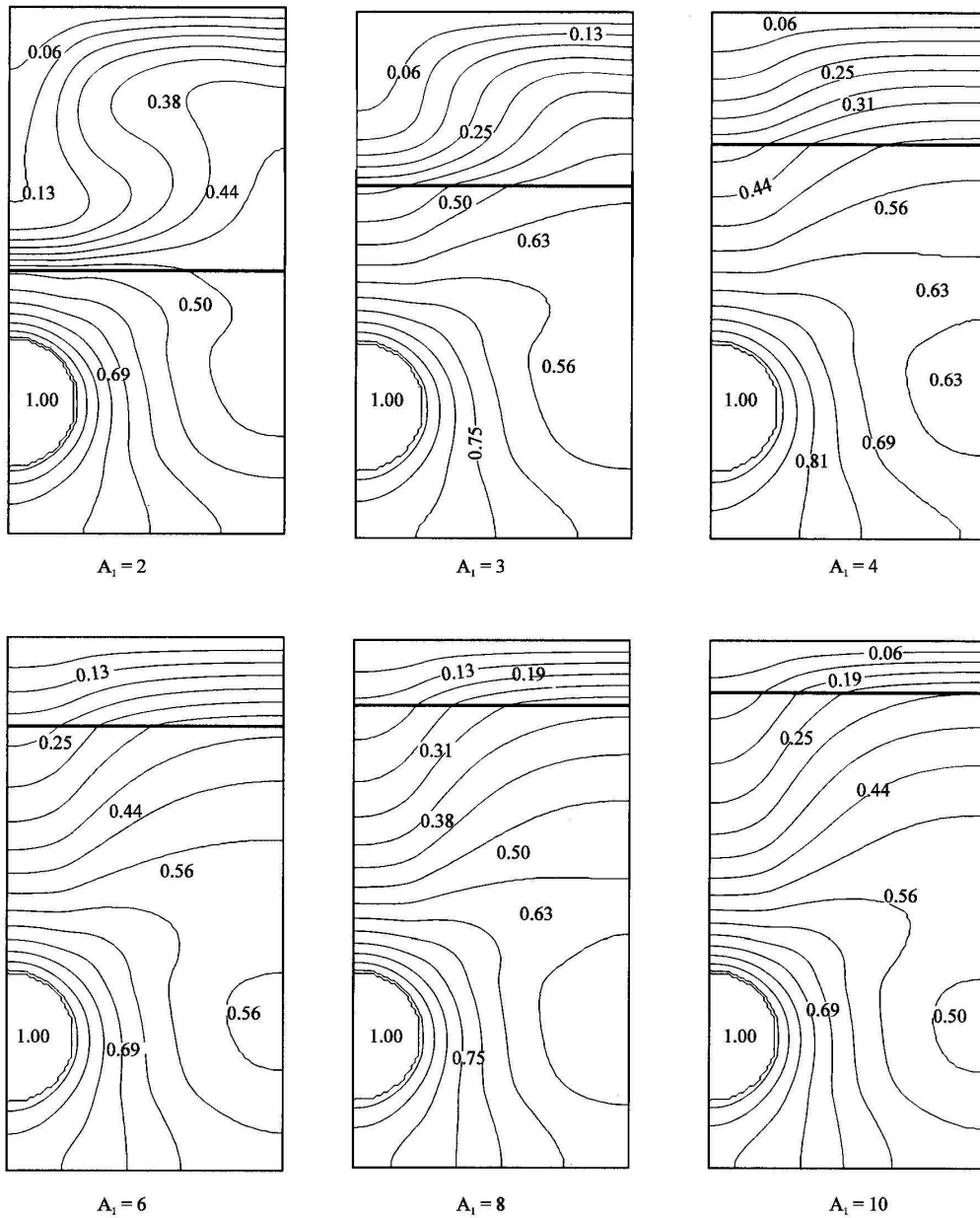
Fig. 2: Isotherms for Ra = 10^5 , Pr = 0.71 , A = 4 , Da = 0.002 , \varepsilon = 0.513 , kr = 1
