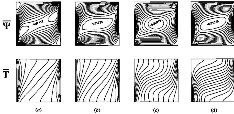
Figure 8. Structures of the mean stream function and the isothermals at Ra = 200 and Ra_v = 500 , with a frequency of (a) 1, (b) 10, (c) 25, and (d) 100.
