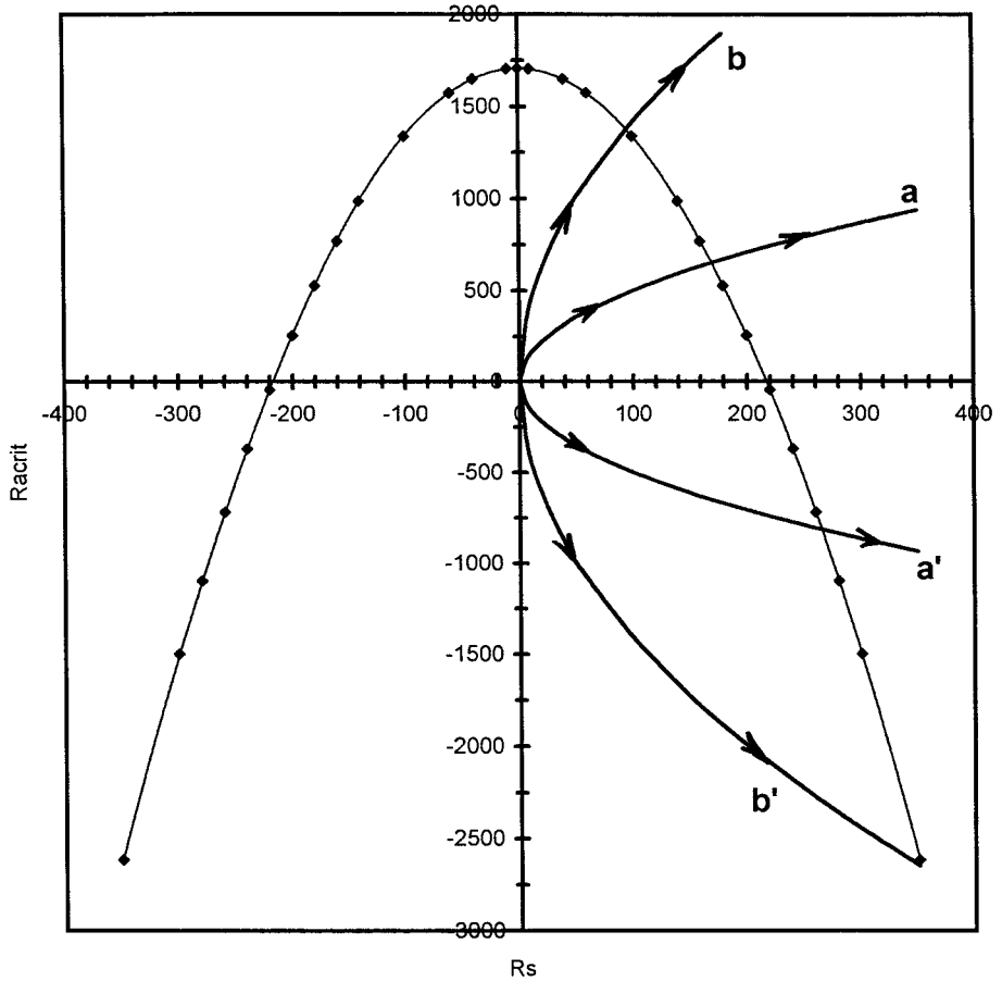
Fig. 1. Variation of Ra_T^{crit} with Ra_S for Le = 100 .
