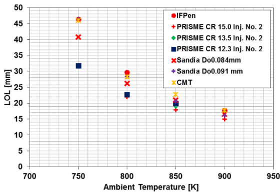
Fig. 7. Measured LOL versus ambient gas temperature for different CR compared to previous results [...].
