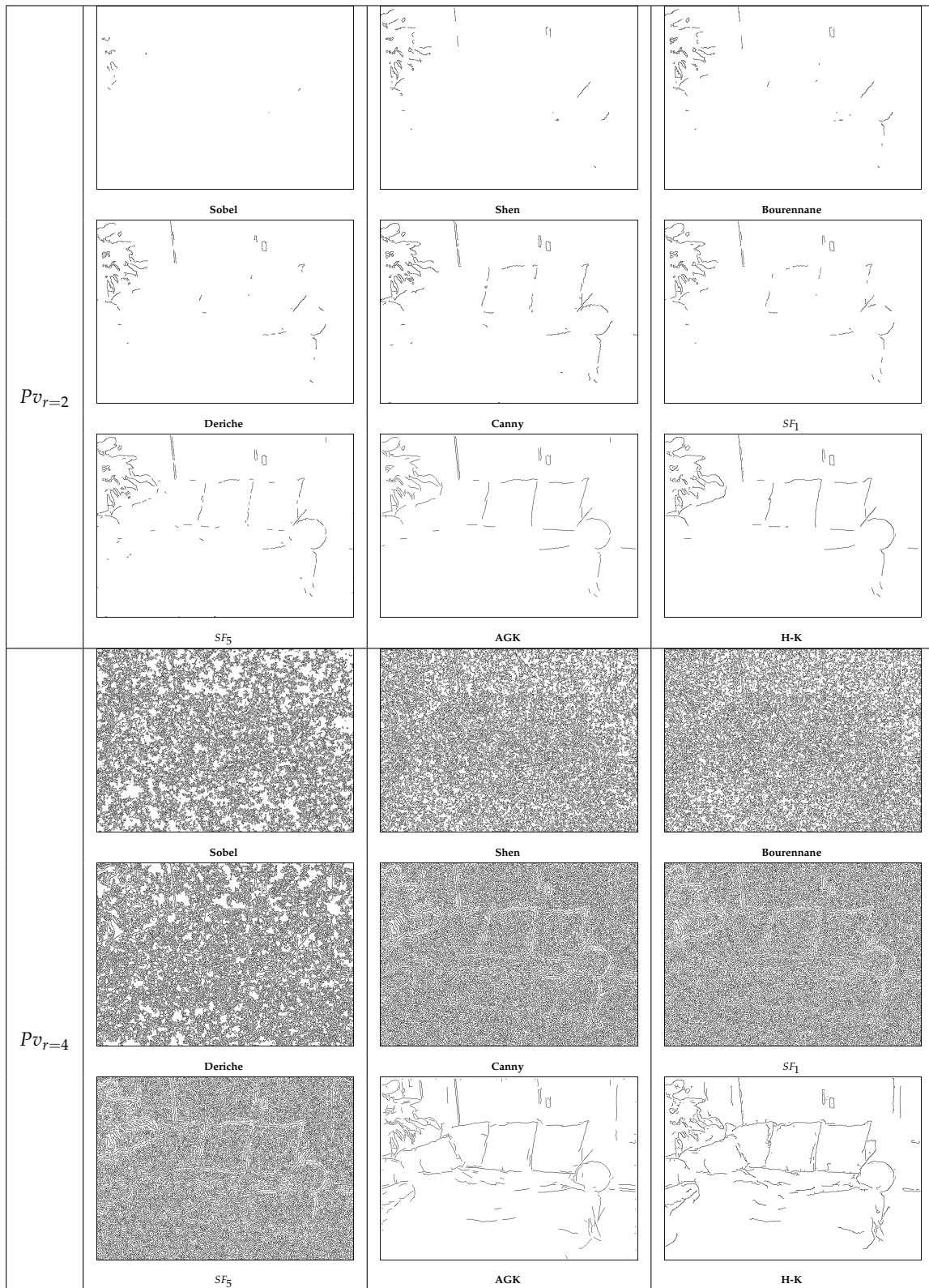
Figure 24. Ideal segmentations for several edge detectors on image 109, PSNR = 14 dB.
