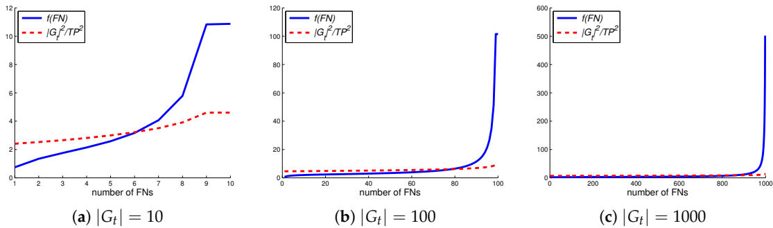
Figure 14. Several examples of f function evolution as a function of the FN number.
