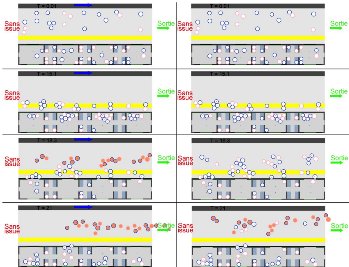
Fig. 7 Photograms of one typical simulation of the platform/train passenger interchange with (on the left) and without (on the right) arrow sign (time stations t=0.01s , 15.1s , 18.3s , 21s ).
