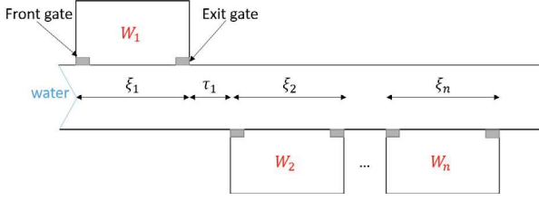
Fig. 1. River-tanks system
