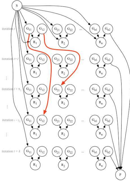
Fig. 3. Extended graph associated to the sub-problem
