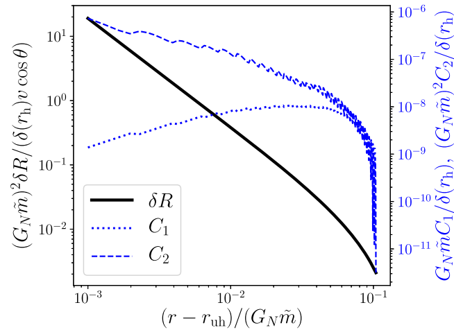
FIG. 2. \mathcal{O}(v) contribution to the Ricci scalar (left axis) and constraint violations (right axis) near the universal horizon, as a function of distance from the latter. The results are in the spin-0 frame, for the solution regular at both the matter and spin-0 horizons. The theory's parameters are \alpha = 0.02 , \beta = 0.01 , and \lambda = 0.1 , corresponding to \alpha' = 0.02 , \beta' = -4.161 , and \lambda' = 4.735 . Note that this solution is not asymptotically flat, as discussed in the text, and that it is determined up to a global rescaling. Because of this, we normalize the \mathcal{O}(v) contribution to the Ricci scalar by the value of \delta at the matter/spin-0 horizon r_h .
