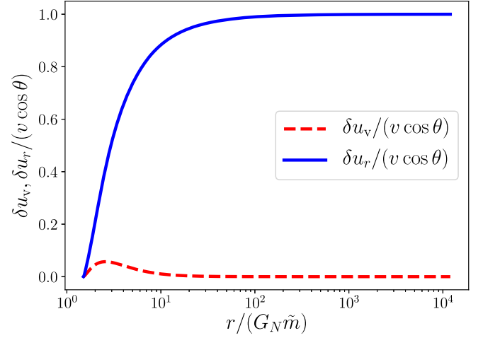
FIG. 4. \mathcal{O}(v) æther perturbations \delta u_\mu for the unique regular solution of the \alpha = \beta = 0 case, outside the universal/spin-0 horizon.
