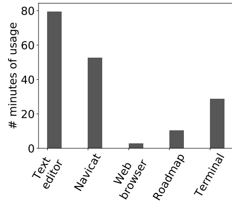
Fig. 4: Time spent using each tool during the 3 development sessions. Periods of inactivity are removed from the plot since no tool is used during those.
