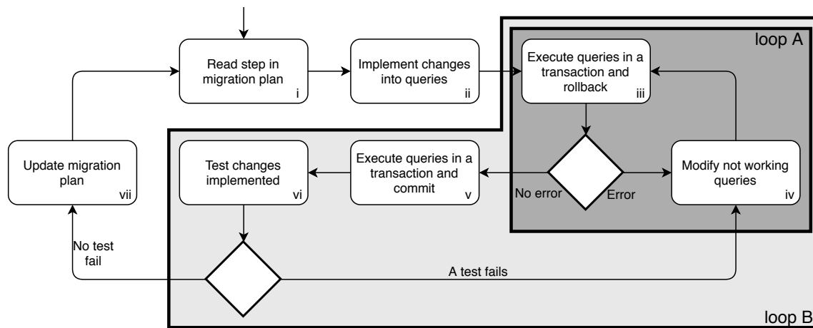
Fig. 2: Process formalized from the database architect actions
