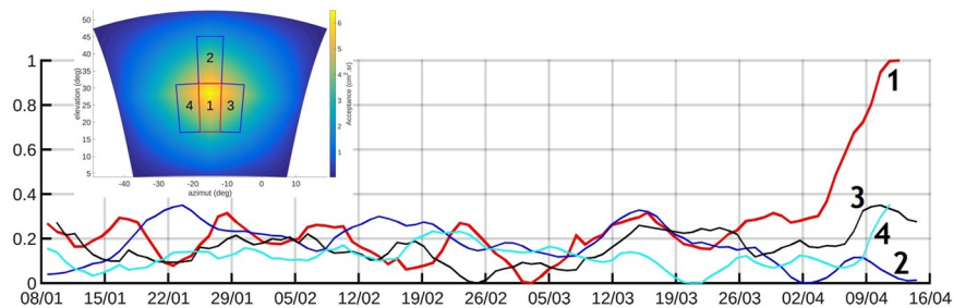
Figure 4. Time variations of the muons flux across different domains of the lava dome. The red curve is for the bundle of lines of sight covering the seismic source zone of Fig. 3. The other three curves are for adjacent areas labeled 2, 3 and 4 in the inset showing the acceptance function of the telescope's view-field. Oscillation amplitudes are arbitrarily set to a common value. The total acceptance of bundles of lines of sight crossing the source area 1 is 54.3 \text{ cm}^2\text{sr} . The acceptances of the merged lines of sight in the areas 2, 3 and 4 are respectively 34.8 \text{ cm}^2\text{sr} , 40.3 \text{ cm}^2\text{sr} , and 45.8 \text{ cm}^2\text{sr} . For comparison, the maximum acceptance of the axial line of sight of the telescope equals 6.5 \text{ cm}^2\text{sr} .
