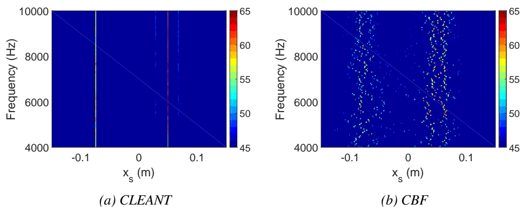
Figure 4: Comparison of deconvolution output for white noise moving sources.
