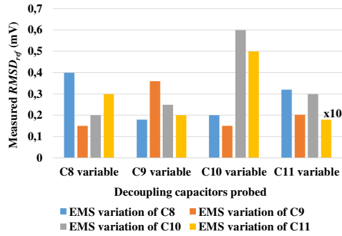
Fig. 9. b. RMSD of the measured FFT amplitude of the magnetic signatures in each case where the value of one input capacitor is changed separately
