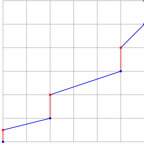
FIGURE 1. The path C_f of f \in \mathbf{Q}_v(\mathbb{I})
