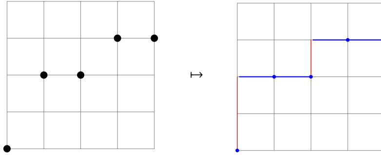
FIGURE 2. The correspondence sending f to R_\iota(f)
