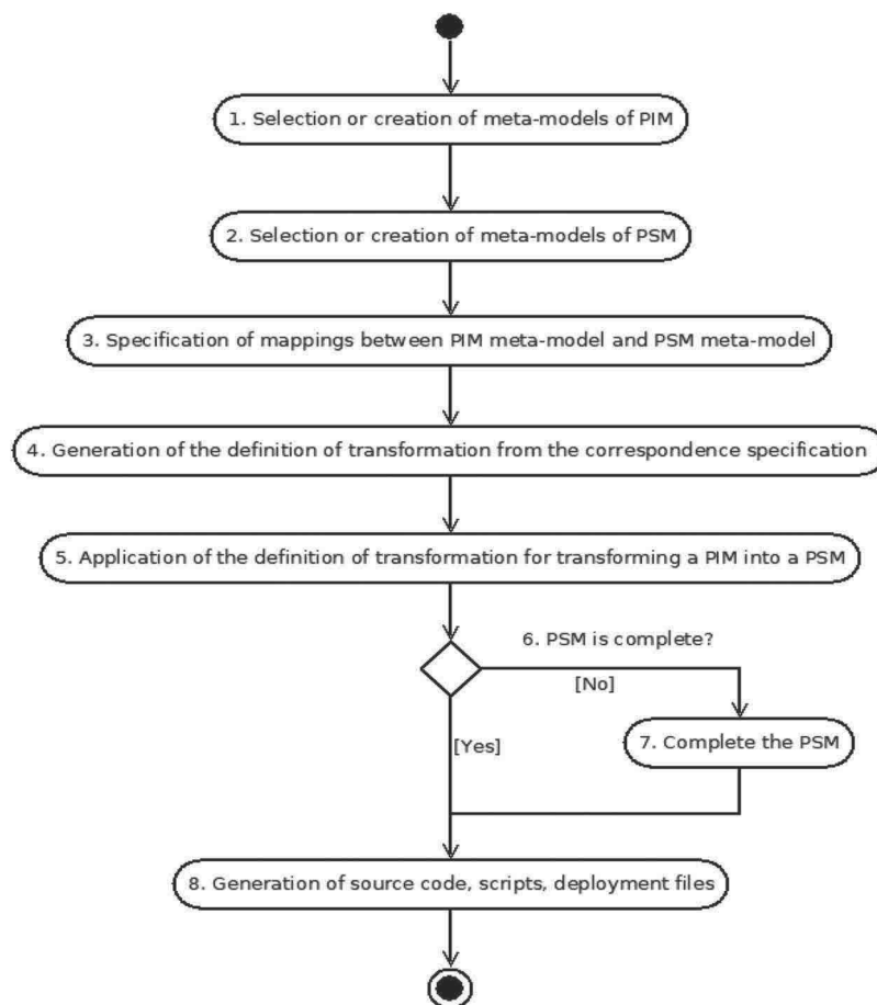
Figure 5. Methodology adopted: activity diagram for the application of the MDA approach.
