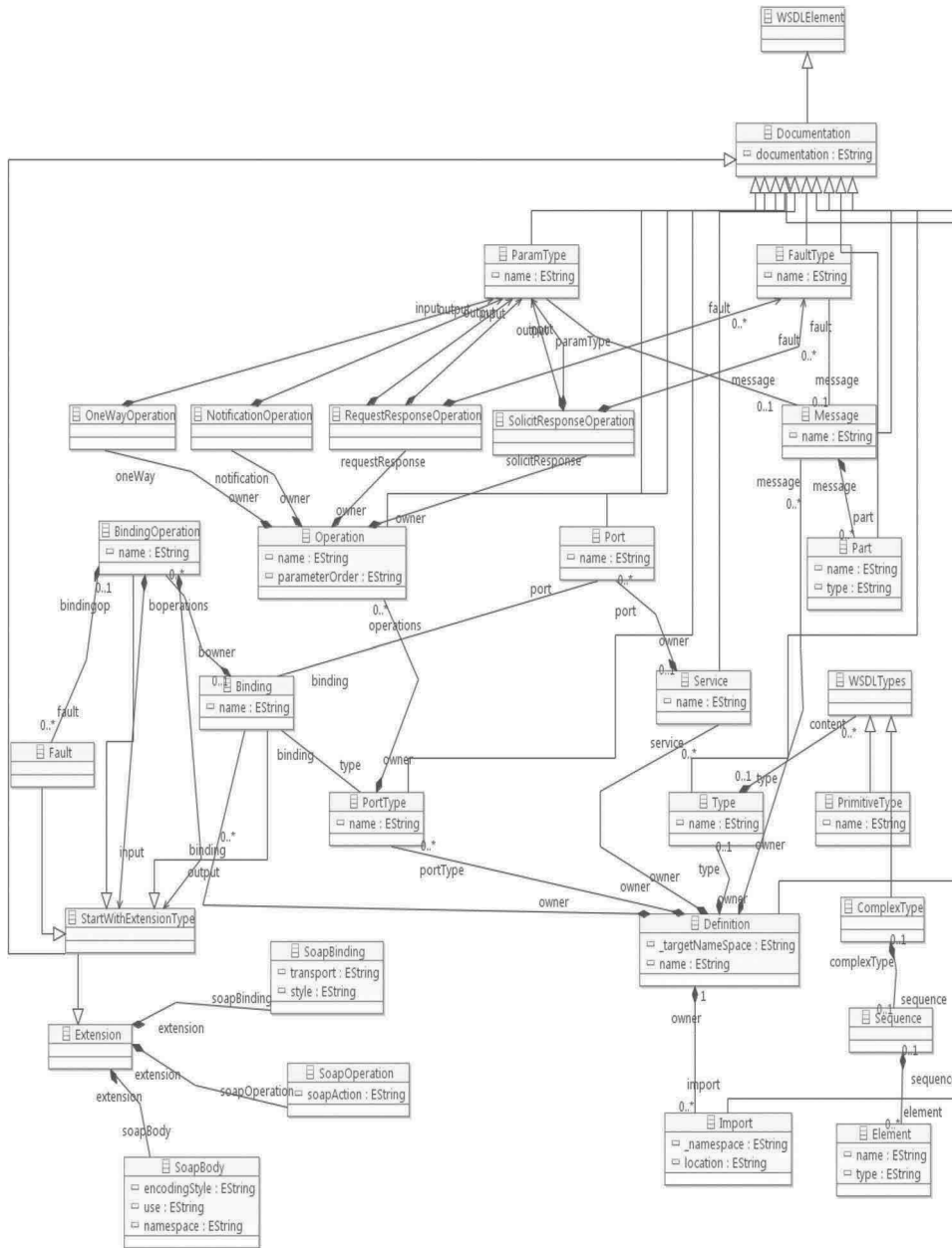
Figure 7. The WSDL metamodel.
