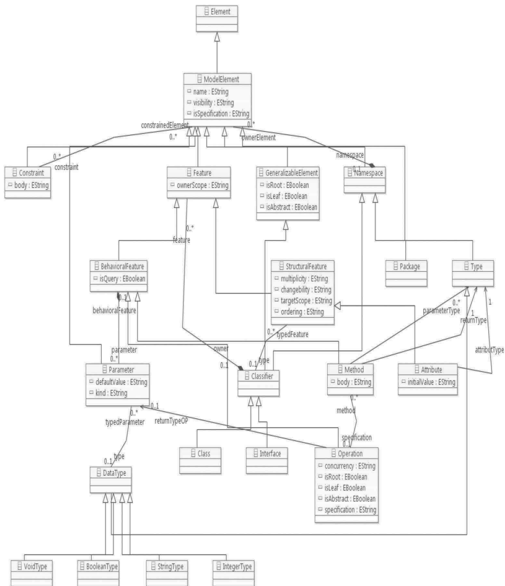
Figure 6. The UML metamodel.
