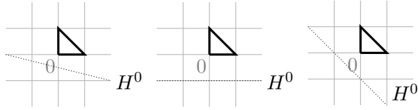
Figure 3: The polytopes \tilde{Q}^0 in the cases where a_1 = 1 and a_2 = 2 , a_1 = 0 and a_2 = 1 and a_1 = a_2 = 1 respectively
