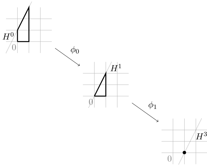
Figure 11: The Log MMP described by the polytopes \tilde{Q}^\varepsilon in the case where n = 2 , a_1 = 2 and \alpha_1 is trivial.
