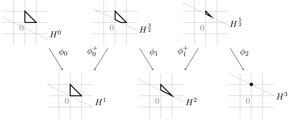
Figure 4: The Log MMP described by the polytopes \tilde{Q}^\epsilon in the case where n = 2 , a_1 = 1 , a_2 = 2 and \alpha_2 is not trivial.
