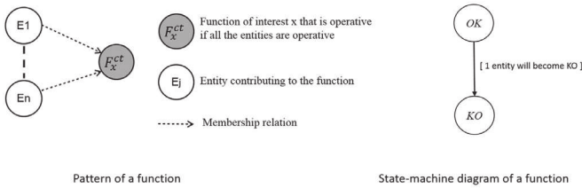
Fig. 6. Pattern and state-machine diagram of a function.
