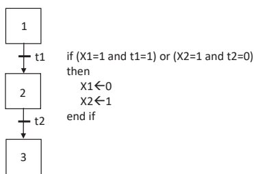
Figure 10. Algorithm of sequential programming.
