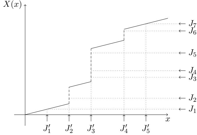
Figure 4: Construction of a random Poisson-box partition C , with subordinator X and arrival times (J_j, j \geq 1) , satisfying C_{\lfloor \cdot \rfloor} = \{\{1\}, \{2\}, \{3, 4, 5\}, \{6\}, \{7\}\}
