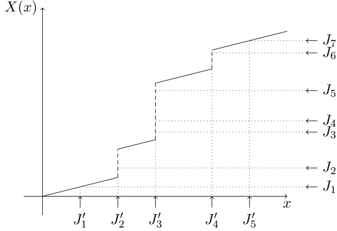
Figure 4: Construction of a random Poisson-box partition C , with subordinator X and arrival times (J_j, j \geq 1) , satisfying C_{|[7]} = \{\{1\}, \{2\}, \{3, 4, 5\}, \{6\}, \{7\}\}
