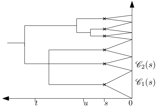
Figure 5: Symbolic representation of the genealogy
