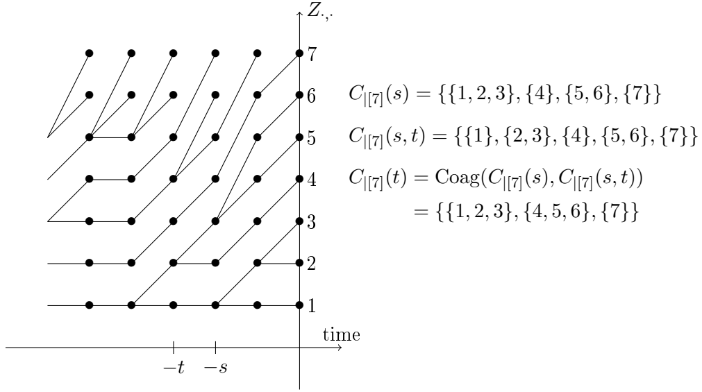
Figure 3: Monotone labelling of an immortal Galton-Watson forest and its consecutive coalescent
