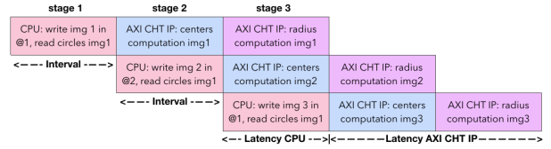
Fig. 7. System Pipeline
