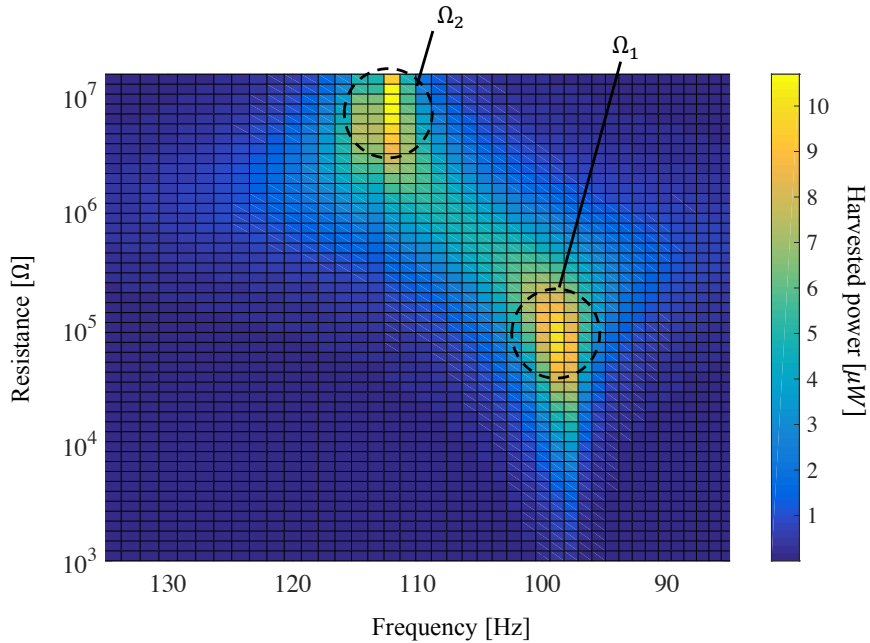
Fig. 14. Experimental harvested power in the (R, f) plane with C = 0\text{nF}
