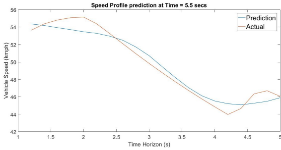
Fig. 15. Use Case 2: Vehicle Speed Profile prediction at time = 5.5 secs
