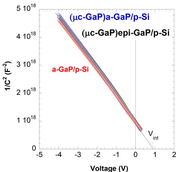
Figure 6. High frequency (100 kHz) 1/C^2 curves versus voltage for n-GaP/p-Si heterostructures with a-GaP (a-GaP and \mu c-GaP layer) and epi-GaP interfaces measured at room temperature.
