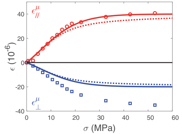
Fig. 4. \Delta E effect for an iron-cobalt alloy: longitudinal and transverse magnetostriction strain as a function of the applied stress \sigma (uniaxial), modelling (lines) and experimental (points) results from reference [35]. The dotted line reproduces the modelling results obtained in reference [35]. The plain line shows the results from equation (26) (modelling parameters: \lambda_s = 40 \times 10^{-6} , \alpha = 1.25 \times 10^{-7} Pa ^{-1} ).
