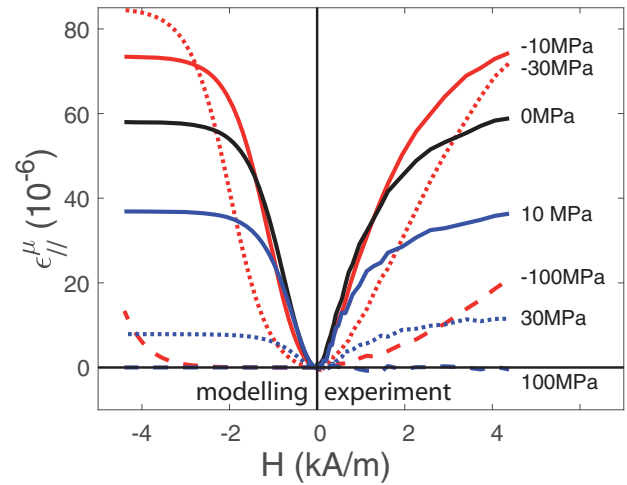
Fig. 2. Longitudinal magnetostriction strain under uniaxial stress for an iron–cobalt alloy: analytical model (left) and experimental results from reference [36] (right) (modelling parameters: \lambda_s = 58 \times 10^{-6} , \kappa = 2.2 \times 10^{-3} \text{ m/A} , \alpha = 10^{-7} \text{ Pa}^{-1} ).
