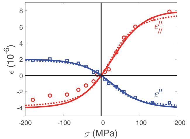
Fig. 5. \Delta E effect for pure iron: longitudinal and transverse magnetostriction strain as a function of the applied stress \sigma (uniaxial), modelling (lines) and experimental (points) results from reference [35]. The dotted line reproduces the modelling results obtained in reference [35]. The plain line shows the results from equation (26) (modelling parameters: \lambda_s = 8 \times 10^{-6} , \alpha = 2.4 \times 10^{-8} Pa ^{-1} ).
