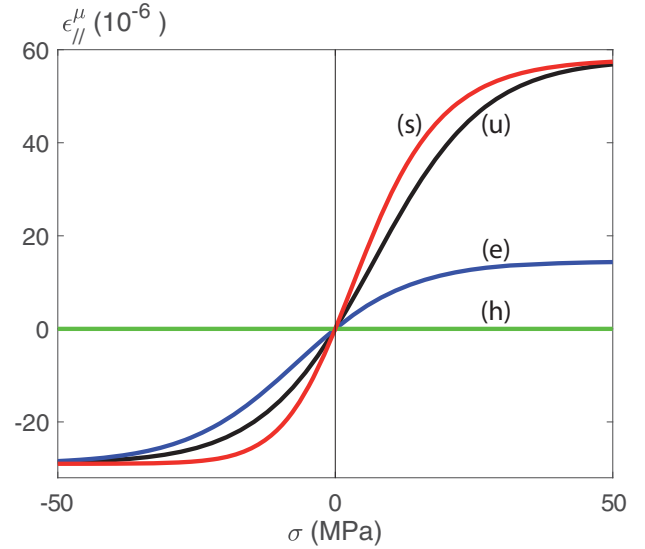
Fig. 1. Magnetostriction strain (maximum principal strain) under no applied magnetic field as a function of stress intensity for uniaxial (u), equibiaxial (e), hydrostatic (h) and pure shear (s) stress states (modelling parameters: \lambda_s = 58 \times 10^{-6} , \kappa = 2.2 \times 10^{-3} \text{ m/A} , \alpha = 10^{-7} \text{ Pa}^{-1} ).
