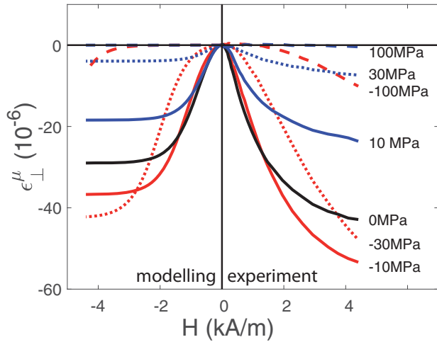
Fig. 3. Transverse magnetostriction strain under uniaxial stress for an iron-cobalt alloy: analytical model ( left ) and experimental results from reference [36] ( right ) (modelling parameters: \lambda_s = 58 \times 10^{-6} , \kappa = 2.2 \times 10^{-3} m/A, \alpha = 10^{-7} Pa ^{-1} ).
