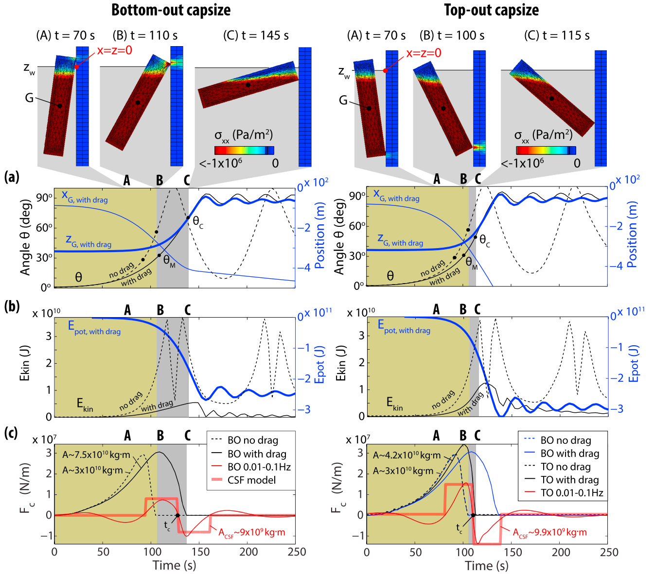
Figure 4. Results of bottom-out (left) and top-out (right) capsizes simulations for an iceberg with \epsilon = 0.2 and H = 800 m. Top images illustrate capsizes motions at different time steps: (A) when the iceberg is accelerating, (B) when the contact force with the wall is maximum, and (C) when at the loss of the iceberg-wall contact. The color scale represents the stress component \sigma_{xx} and is saturated beyond -1 \times 10^6 Pa, to simplify the illustration. Variations with time of (a) angle of rotation ( \theta , black curve) and coordinates x_G and z_G of the center of mass G (blue), (b) iceberg kinetic ( E_{kin} , black) and potential ( E_{pot} , blue) energies, and (c) horizontal force density ( F_c , black) and corresponding 0.01-0.1 Hz band-pass filtered force (red). The red thick curve shows the CSF model that best fits the force in the seismic band. In each graph, dashed curves represent time series of \theta , E_{kin} and F_c when water drag is not accounted for. Gray-shaded boxes indicate the time range when the iceberg is in contact with the wall (i.e., F_c > 0 N and \theta \leq \theta_C ). Same for yellow boxes but for capsizes simulations without drag. \theta_M and \theta_C in (a) indicate the angles for maximum contact force and loss of iceberg/wall contact, respectively.
