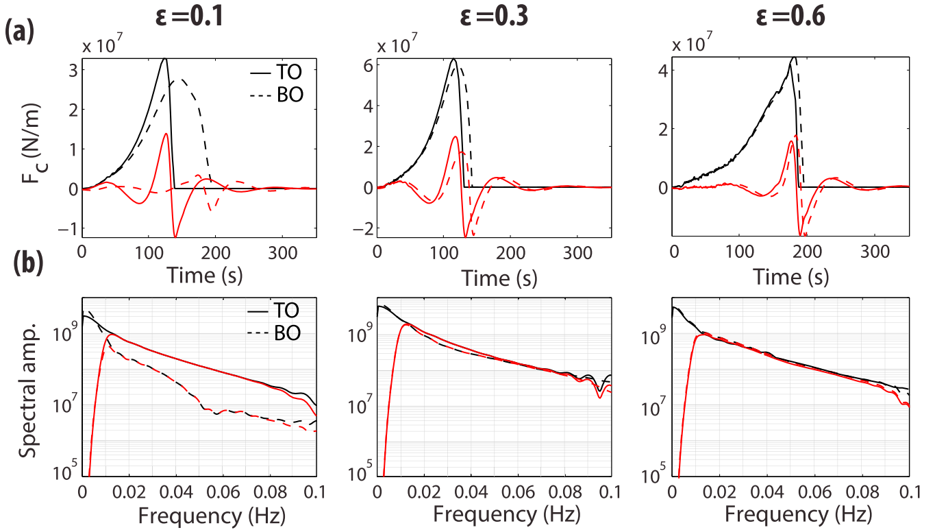
Figure 9. (a) Variations of the force history for TO (solid curves) and BO (dashed curves) icebergs capsizes with \epsilon = 0.1, 0.3 and 0.6 and H = 1000 m. The red curves show the 0.01- to 0.1-Hz filtered forces. (b) Variations of spectral amplitudes with frequency, associated with each force model.
