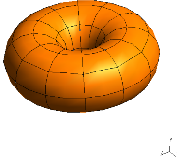
FIGURE 5.1. Computational domain \Omega . Only the macrocells of the mesh are visible. The represented mesh contains 240 macrocells (poloidal refinement set to n_{pol} = 3 and toroidal refinement set to n_{tor} = 3 . In the numerical experiments, we take n_{pol} = 3 and n_{tor} = 5 , which leads to a mesh of 400 macrocells). Each macrocell is then cut regularly into the three directions.
