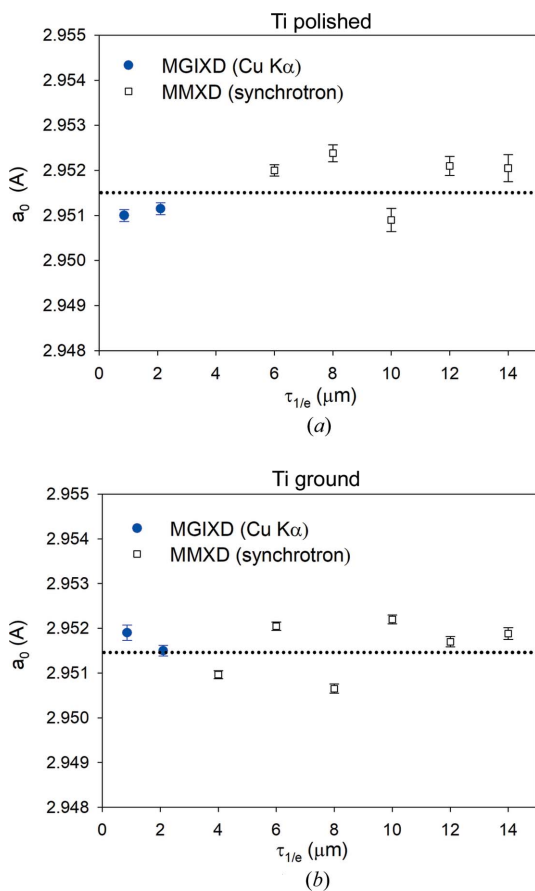
Figure 12 The depth-dependent profile (in the range 0\text{--}14 \mu\text{m} ) of lattice parameter a_0 for (a) polished and (b) ground samples. Comparison of the results from a classical diffractometer (MGIXD) and synchrotron EDDI experiment (MMXD).
