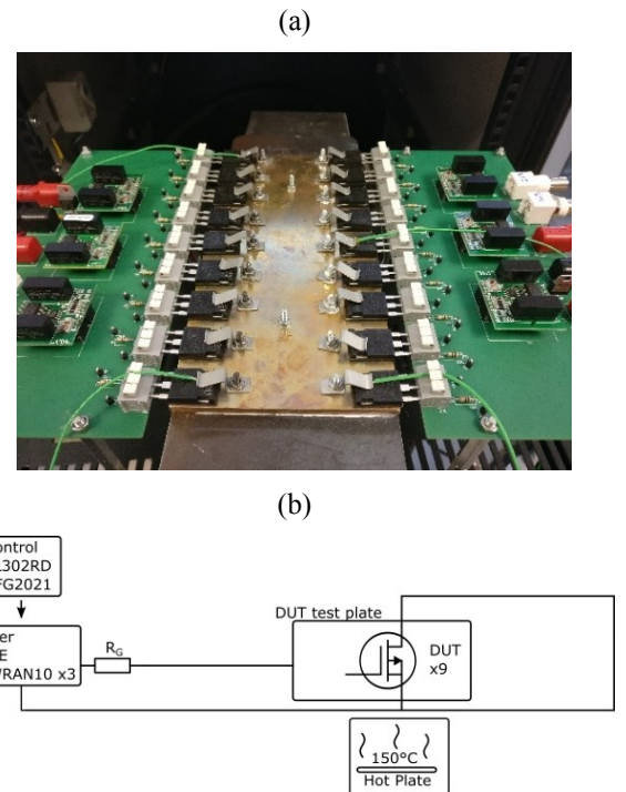
Fig. 1. (a) Ageing setup on the hotplate (tests running at 150°C). 18 MOSFETs (9x2) can be aged simultaneously (b) Scheme of ageing test
