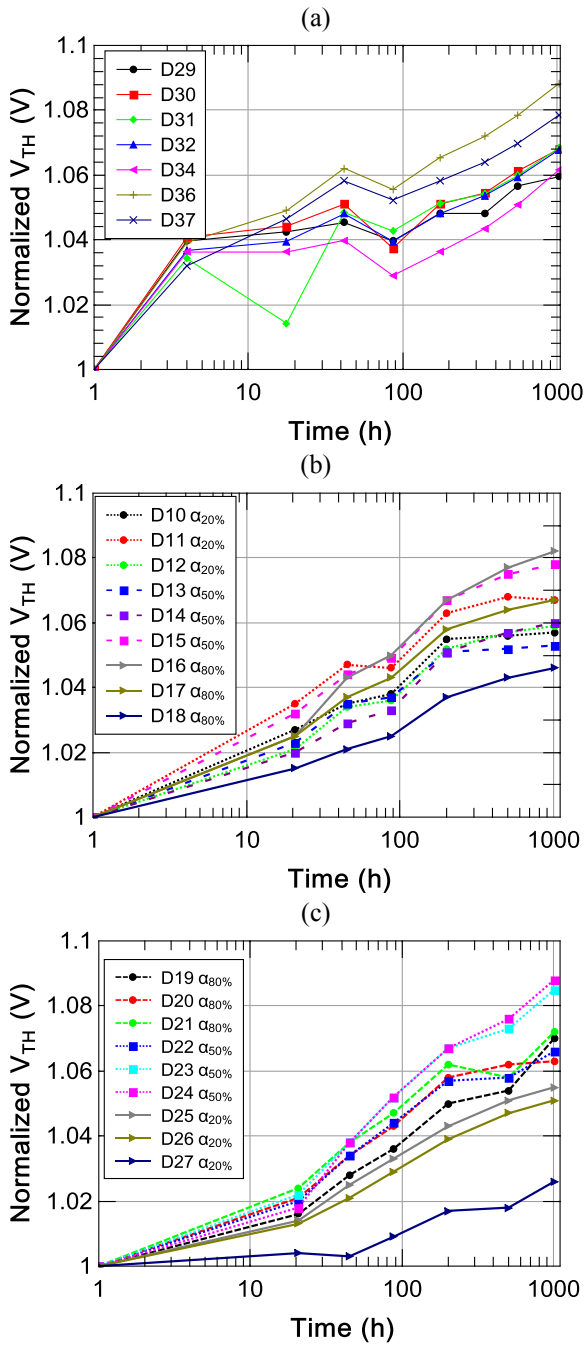
Fig. 6. (a) Normalized threshold voltage shift during HTGS2 static ageing at ambient temperature. (b) Normalized threshold voltage shift during HTGS2 dynamic ageing. (c) Normalized threshold voltage shift during HTGS3 dynamic ageing.
