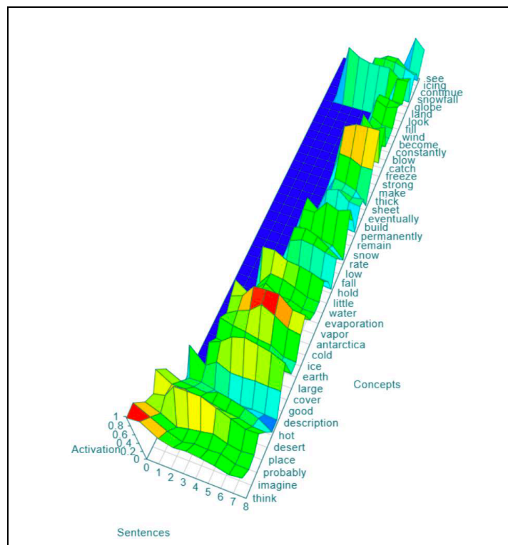
Figure 2. Activation scores provided by AMoC for a sample text.
