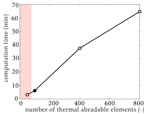
Figure 10. Evolution of the computation time with the number of thermal abrasable coating elements
